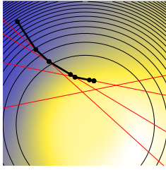
Abbildung 25: Active-Set-Methode
