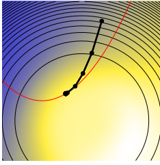
Abbildung 27: Nichtlineare Interior-Point-Methode
