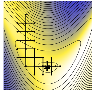
(c) Iteration
