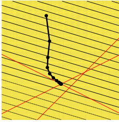
Abbildung 26: Lineare Interior-Point-Methode
