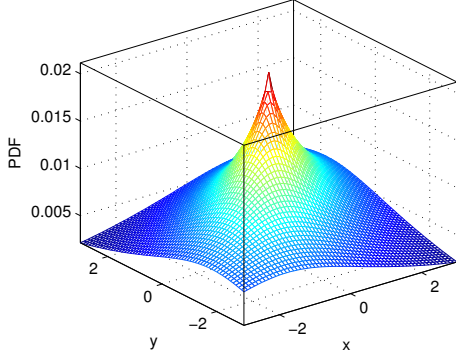
Fig. 1. PDF of MPE_2(\mathbf{0}, \Sigma, 0.4)
