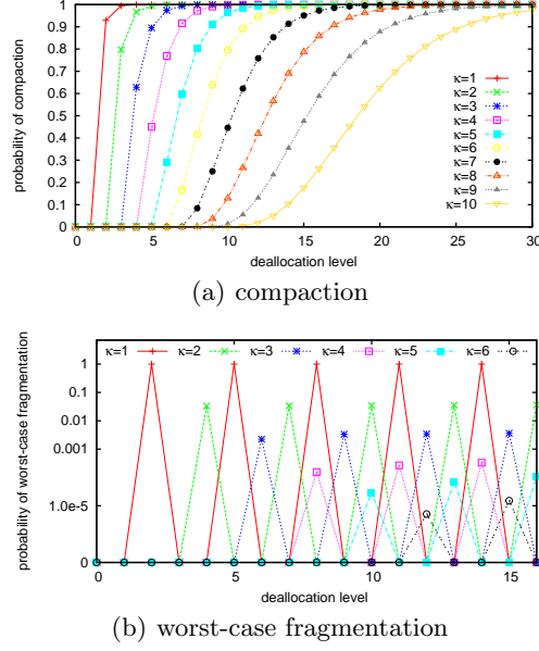
Fig. 4. Probability of reaching compaction and worst-case fragmentation
