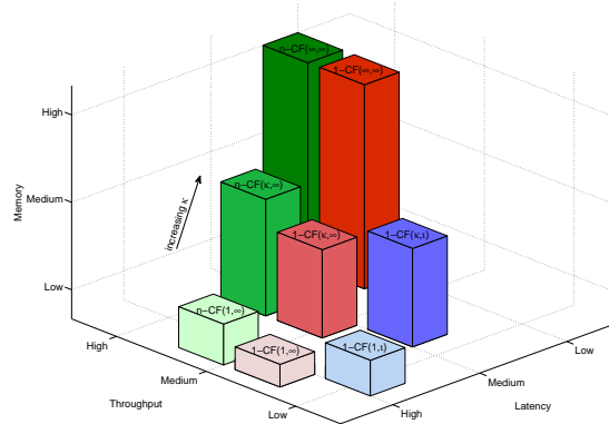
Fig. 1. Deallocation throughput, system latency, and memory fragmentation with different versions and configurations of Compact-fit
