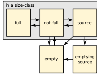
Fig. 5. The lifetime of a page
