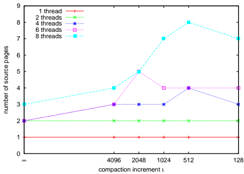
(c) transient size-class fragmentation
