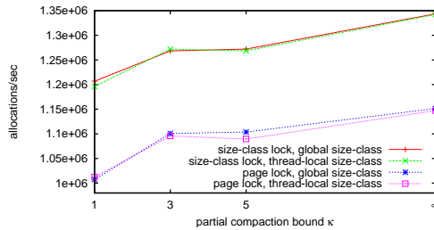
Fig. 8. Allocation throughput of a single thread with decreasing partial compaction
