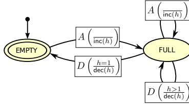
Fig. 3. Size-class automaton with \pi = 1
