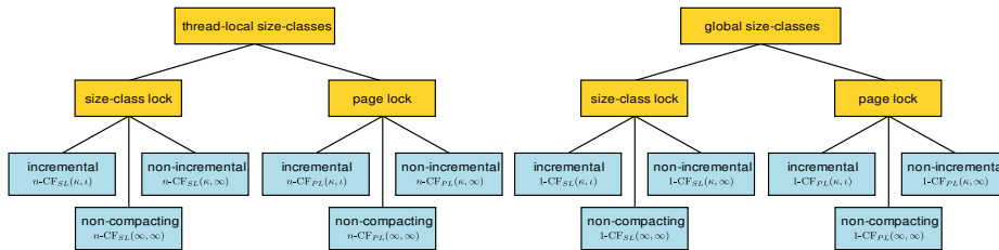
Fig. 7. Concurrent CF versions
