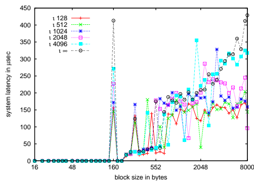
(b) system latency with 8 threads
