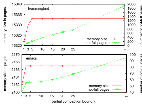
Fig. 11. Memory usage and size-class fragmentation for Hummingbird and Emacs
