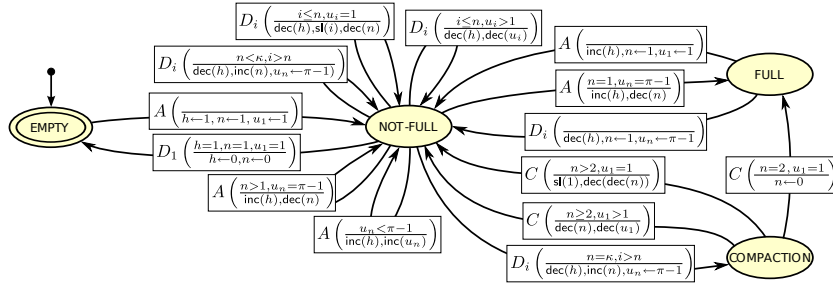
Fig. 2. Size-class automaton with \pi > 1
