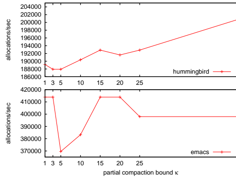
Fig. 10. Allocation throughput for Hummingbird and Emacs
