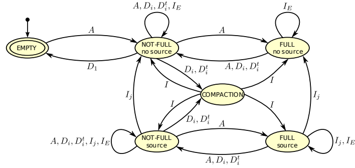
Fig. 6. Incremental size-class automaton with \pi > 1
