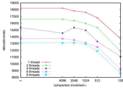
(a) allocation throughput
