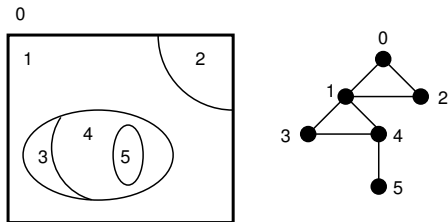
Figure: region adjacency graph
